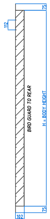
VERTICAL SECTION THROUGH 112 FIXED BLADE LOUVRE W/ 75MM FRONT FLANGE
