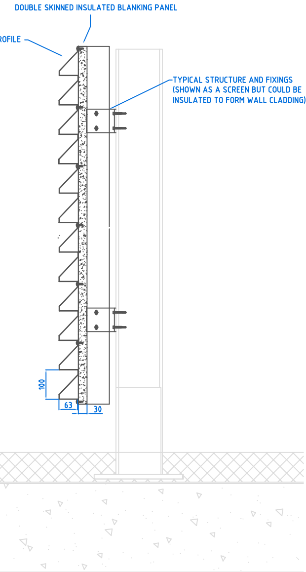
VERTICAL SECTION THRU 2 BLADE DUMMY LOUVRE PROFILE (0.9mm gauge) (SHOWN AS A SCREEN BUT COULD BE INSULATED TO FORM WALL CLADDING)
