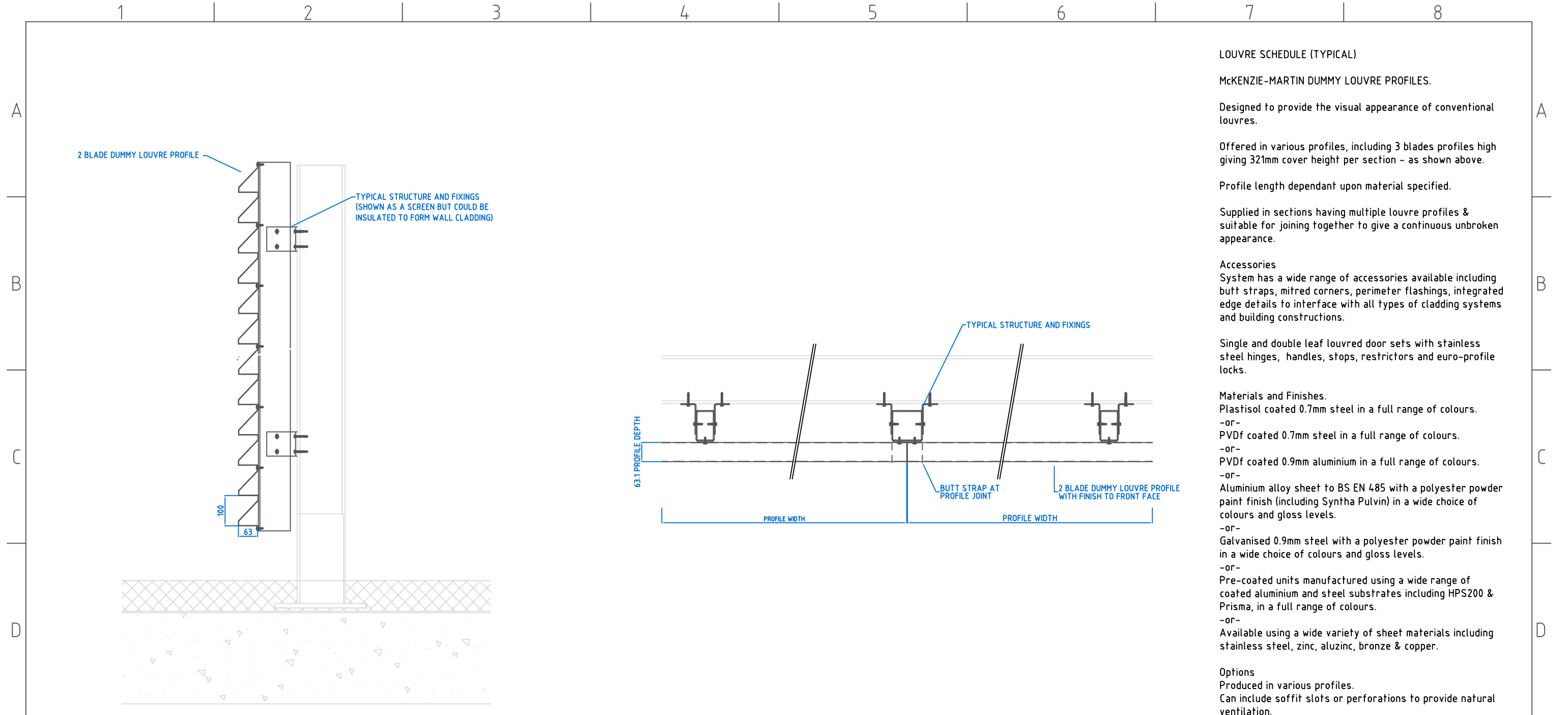
VERTICAL SECTION THRU 2 BLADE DUMMY LOUVRE PROFILE (0.9mm gauge) (SHOWN AS A SCREEN BUT COULD BE INSULATED TO FORM WALL CLADDING)
