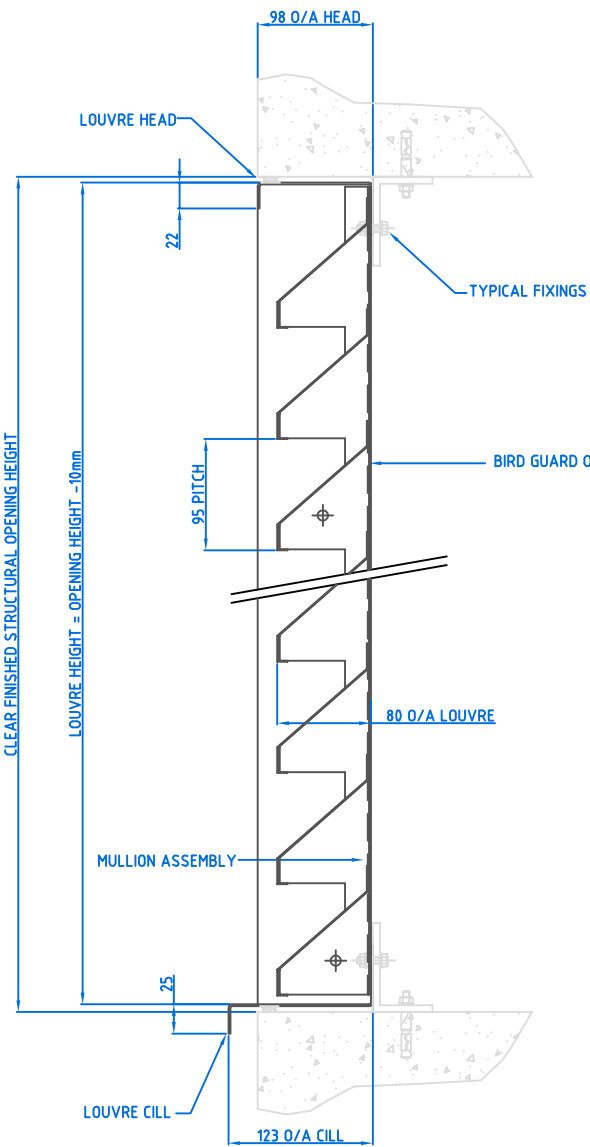
VERTICAL SECTION THRU CONTINUOUS FIXED LOUVRE LOUVRE with 95mm PITCH BLADES
