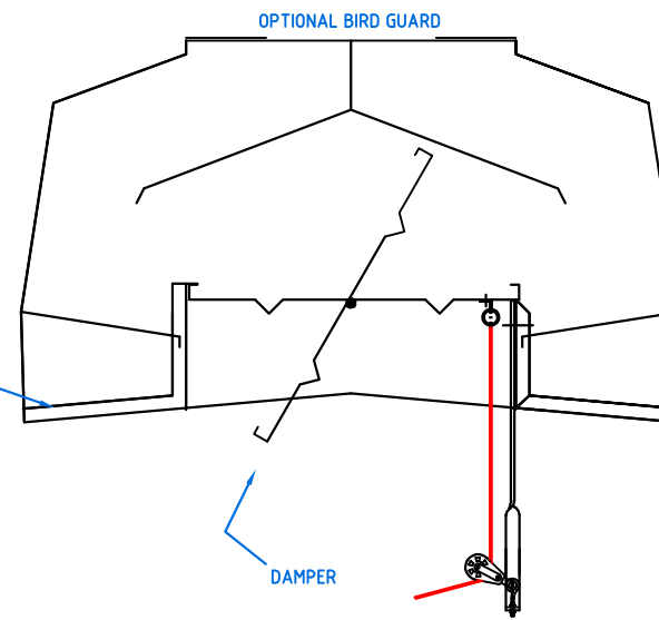
END VIEW CABLE OPERATION
