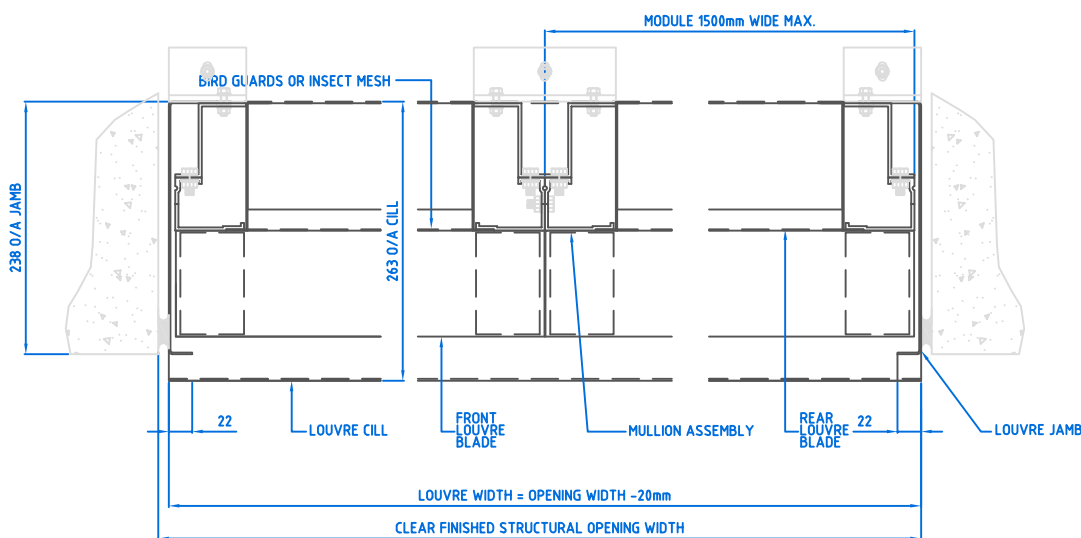
PLAN SECTION THRU Maximair "Inverted" Double Bank 100 LOUVRE
