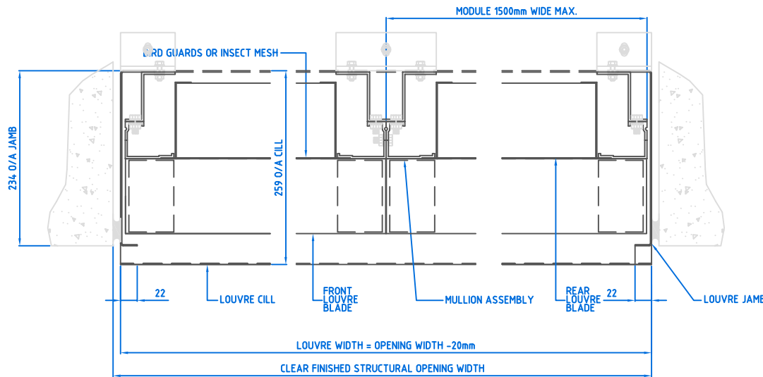
PLAN SECTION THRU Maximair Double Bank 100 LOUVRE
