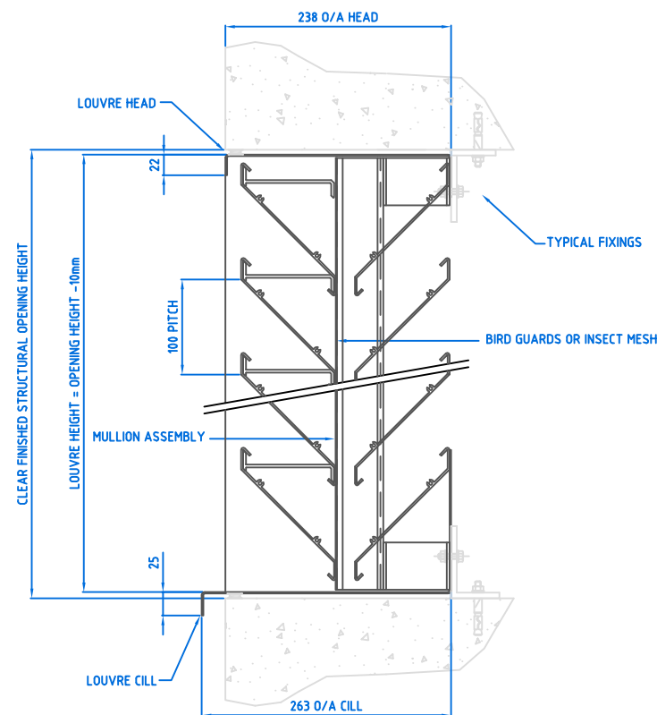
VERTICAL SECTION THRU Maximair "Inverted" Double Bank 100 LOUVRE
