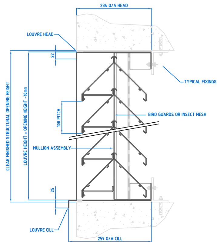
VERTICAL SECTION THRU Maximair Double Bank 100 LOUVRE
