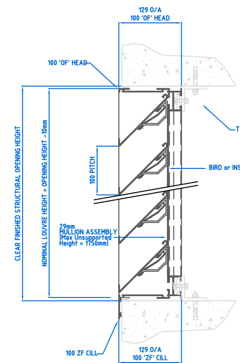
VERTICAL SECTION THRU K Series 100 LOUVRE WITH 'OF' HEAD & 'ZF' CILL
