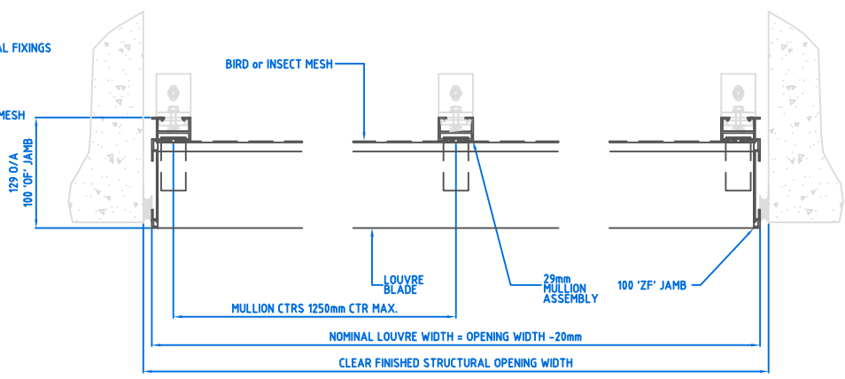
PLAN SECTION THRU K Series 100 LOUVRE WITH 'OF' JAMBS
