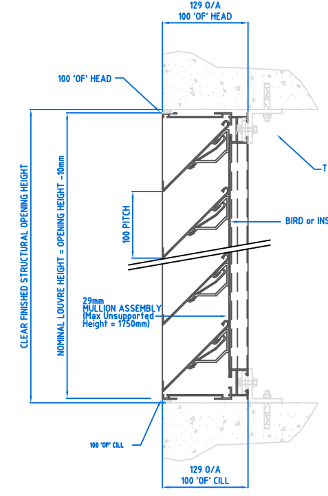
VERTICAL SECTION THRU K Series 100 LOUVRE WITH 'OF' HEAD & CILL
