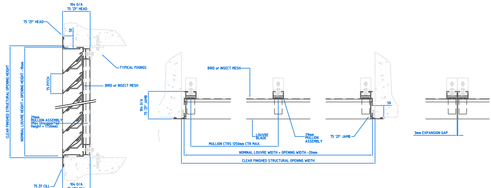
VERTICAL SECTION THRU K Series 75 LOUVRE WITH 'ZF' HEAD & CILL
