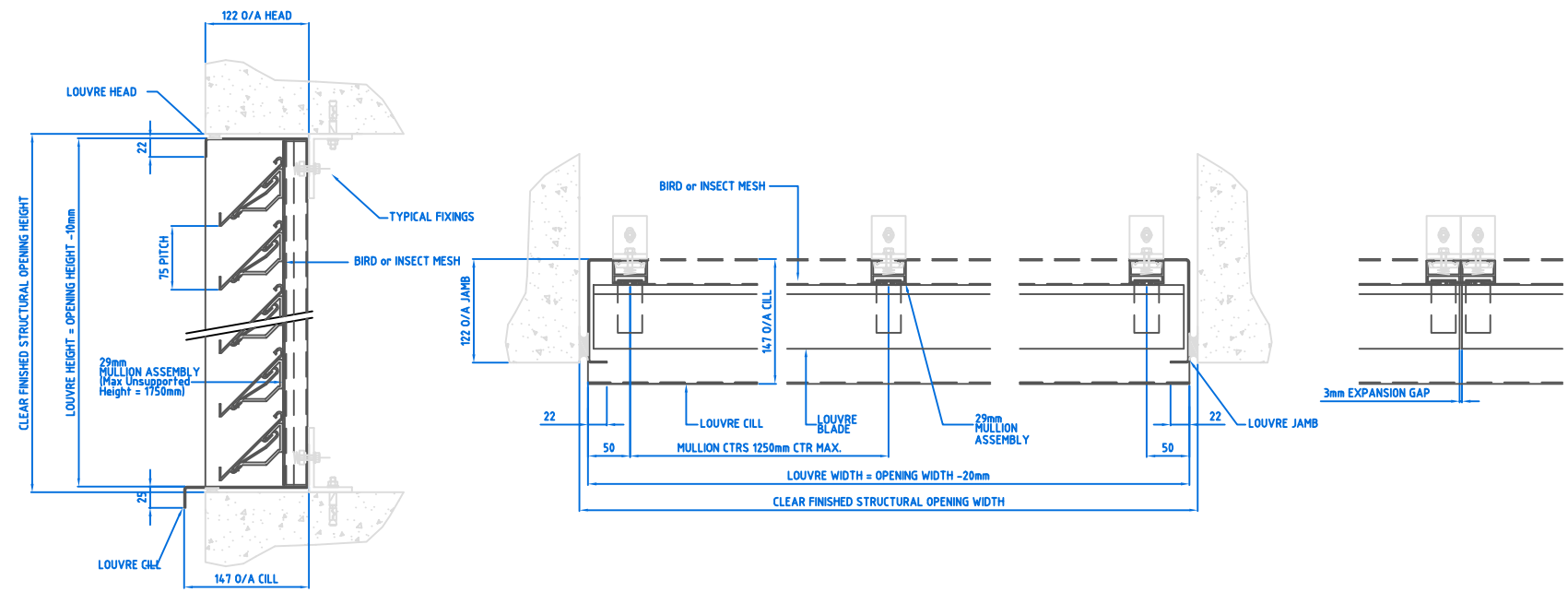
VERTICAL SECTION THRU K Series 75 LOUVRE
