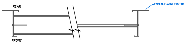
HORIZONTAL SECTION THRU OPERATING BOX LOUVRE SHOWING BLADE IN OPEN & CLOSED POSITION
