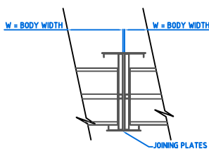
HORIZONTAL JOINT DETAIL BETWEEN LOUVRE MODULES
