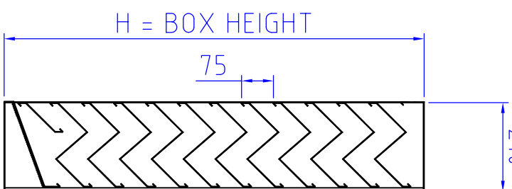
VERTICAL SECTION THROUGH 75MM TRIPLE BANK LOUVRE
