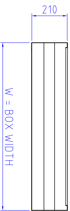
PLAN VIEW OF 75MM TRIPLE BANK LOUVRE
