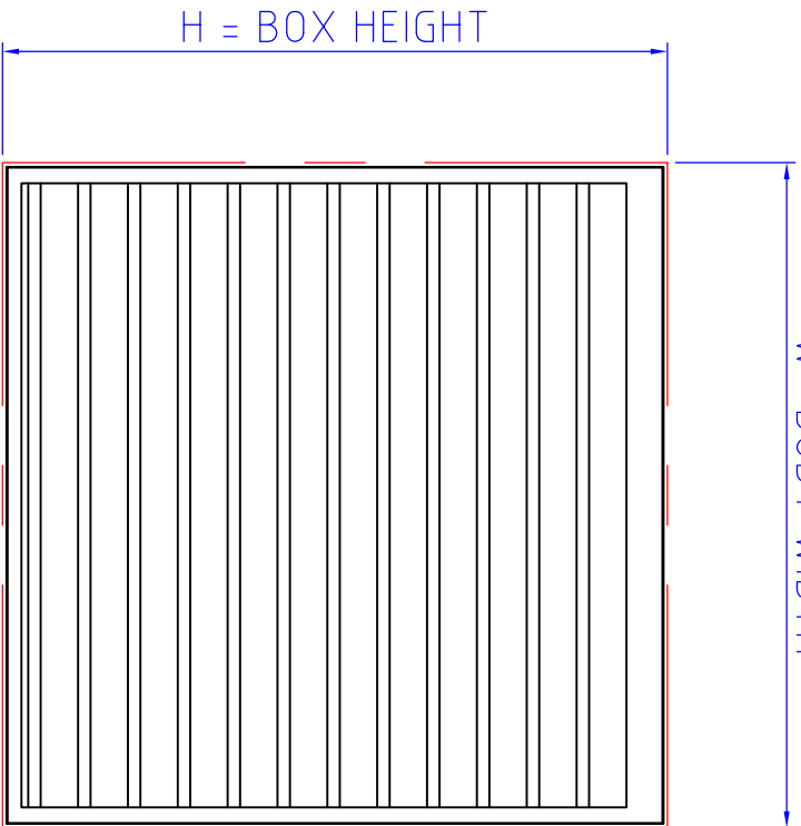
FRONT VIEW 75MM TRIPLE BANK LOUVRE
