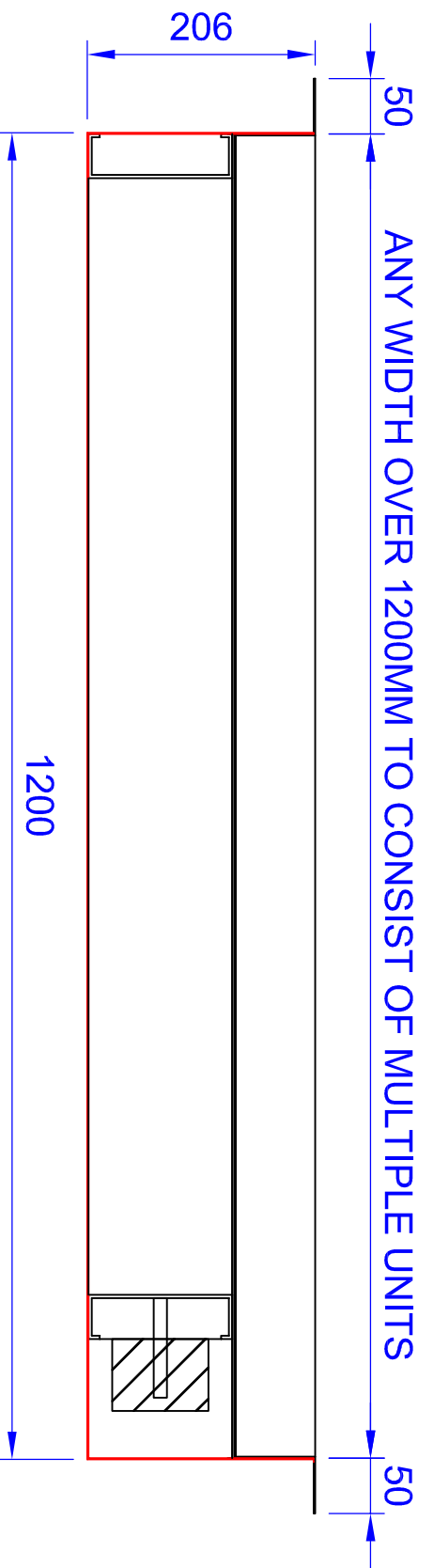
LOUVRE AND DAMPER - PLAN VIEW
