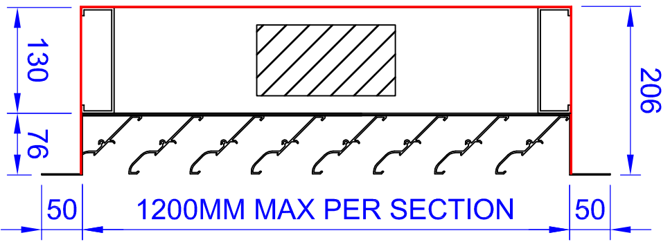
LOUVRE AND DAMPER - ELEVATION
