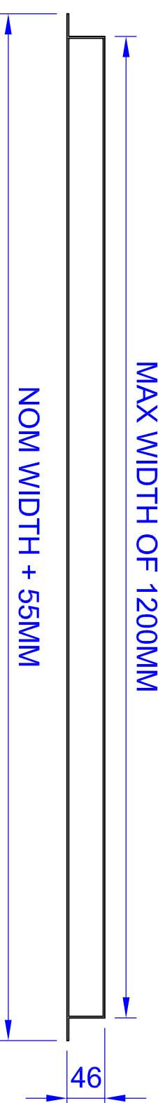
NON-VISION GRILLE - PLAN VIEW
